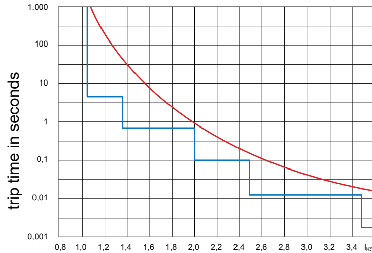
times rated current trip curve
