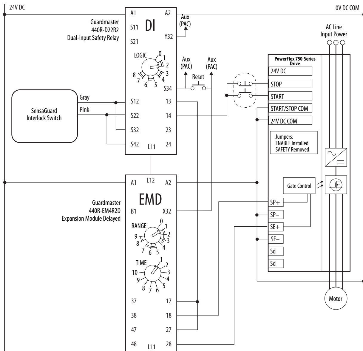
Figure 8 - Stop Category 1
