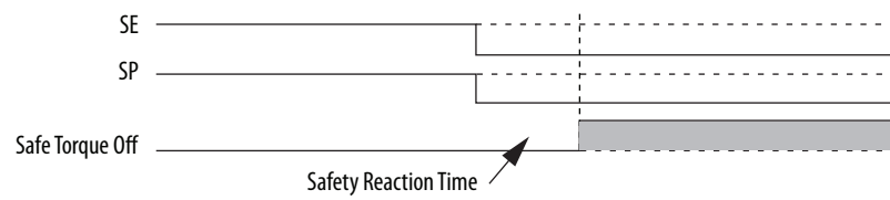
Figure 1 - Safety Reaction Timing Diagram
