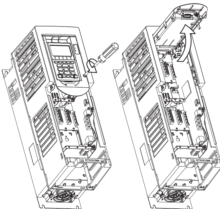
Panel-mounted Drives
