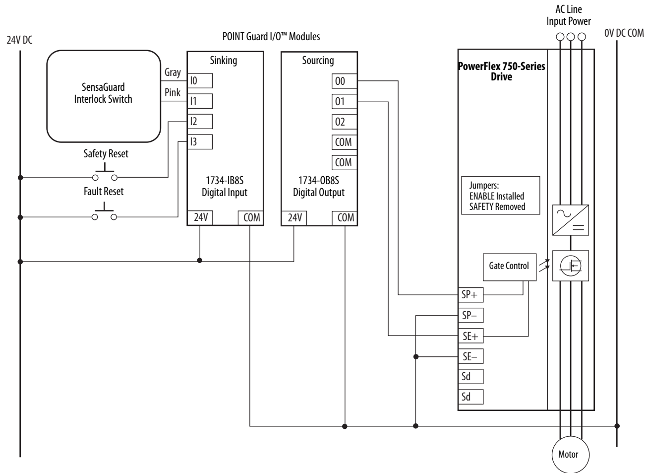
Figure 9 - Stop Category 0
