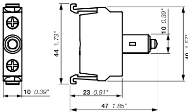
MLBL Dimensions (mm, inches)
