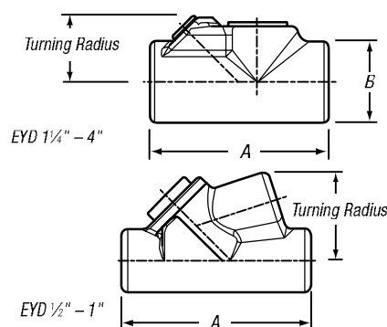
EYD Series Drain Sealing Fittings
