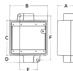
Fig. C through-feed
