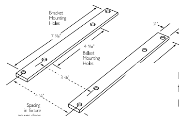
PC-849 Mounting bracket for Fig. 2, 3a, 8, 8a & 10.
