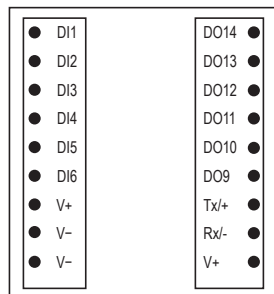
Figure 1. -PM8 Board
