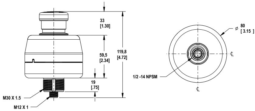
Figure 2. Standard 40 mm Pushbutton
