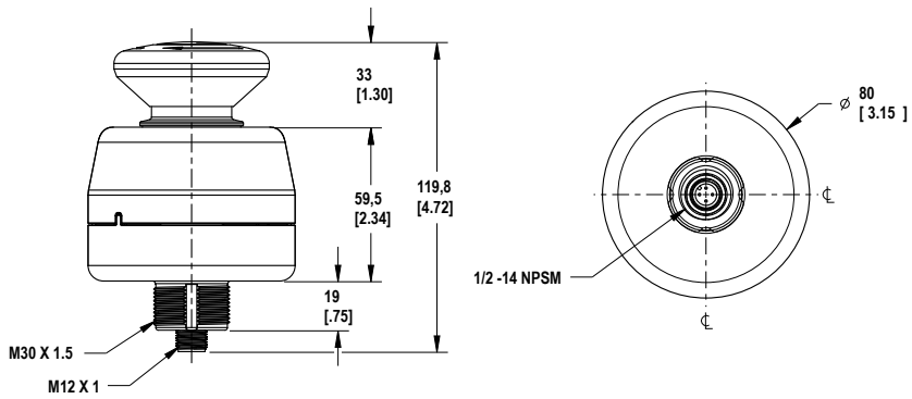
Figure 3. Large 60 mm Pushbutton
