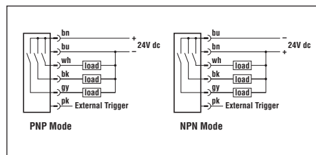
Wiring Diagram
