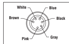
Pin Out Diagram Corresponding to MQCD-Series Quick-Disconnect Cable
