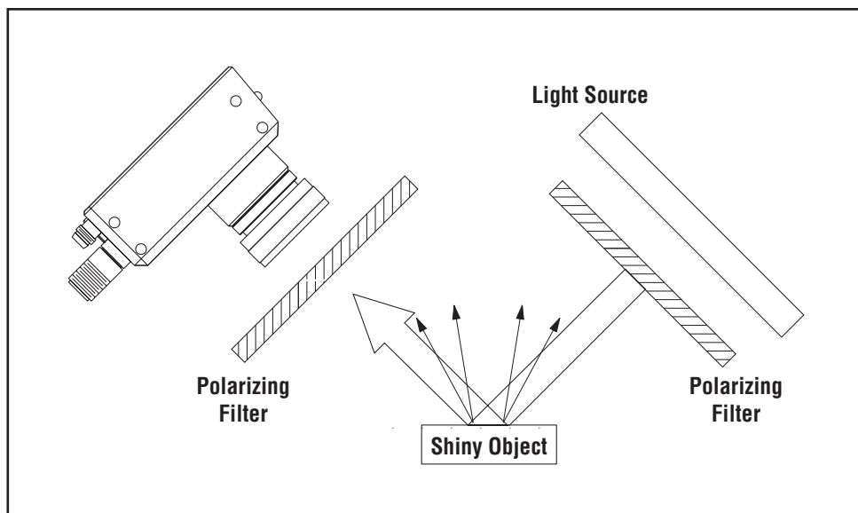
Polarized Light
