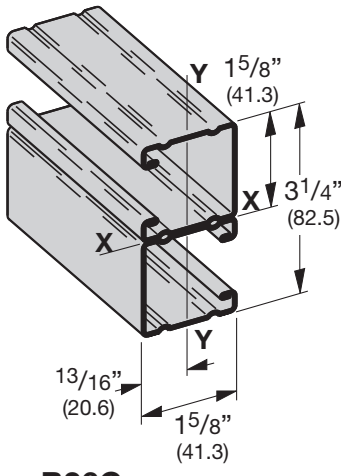
B26C Wt. 2.24 Lbs./Ft. (3.33 kg/m)
