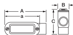
LB Body
