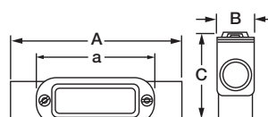
TB Body
