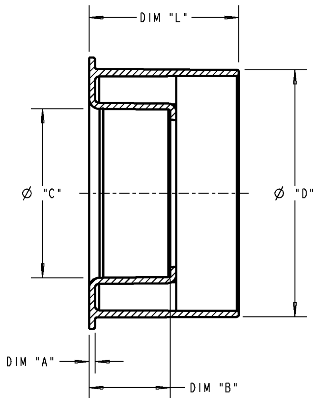
SECTION C-C SCALE 0.750
