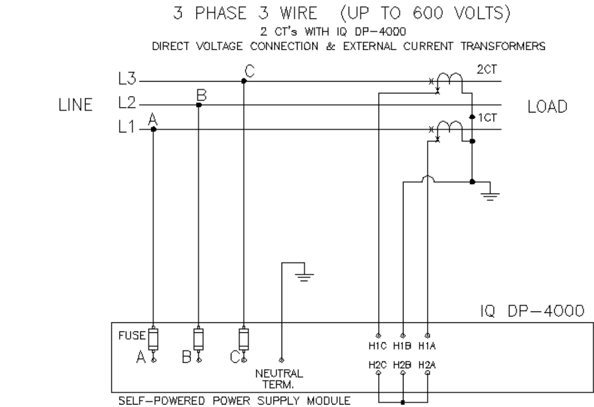
Figure 4.12 3-Phase, 3-Wire (up to 600 volts) Wiring Diagram( 2 CTs)
