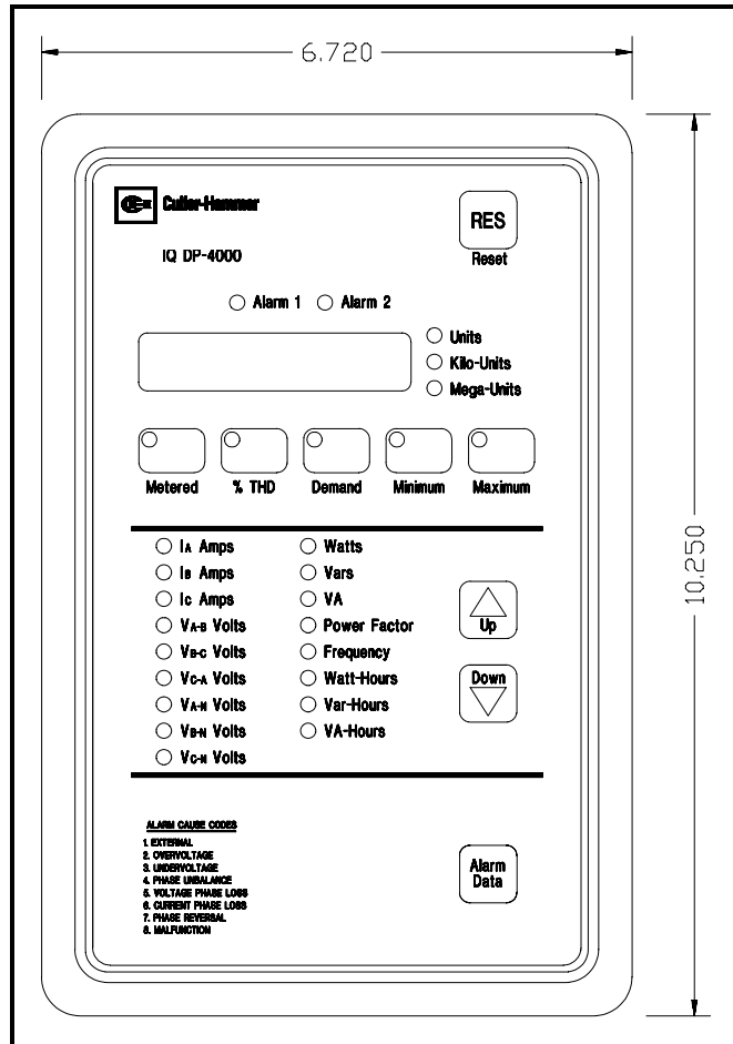
Figure 3.1 Operator Panel
