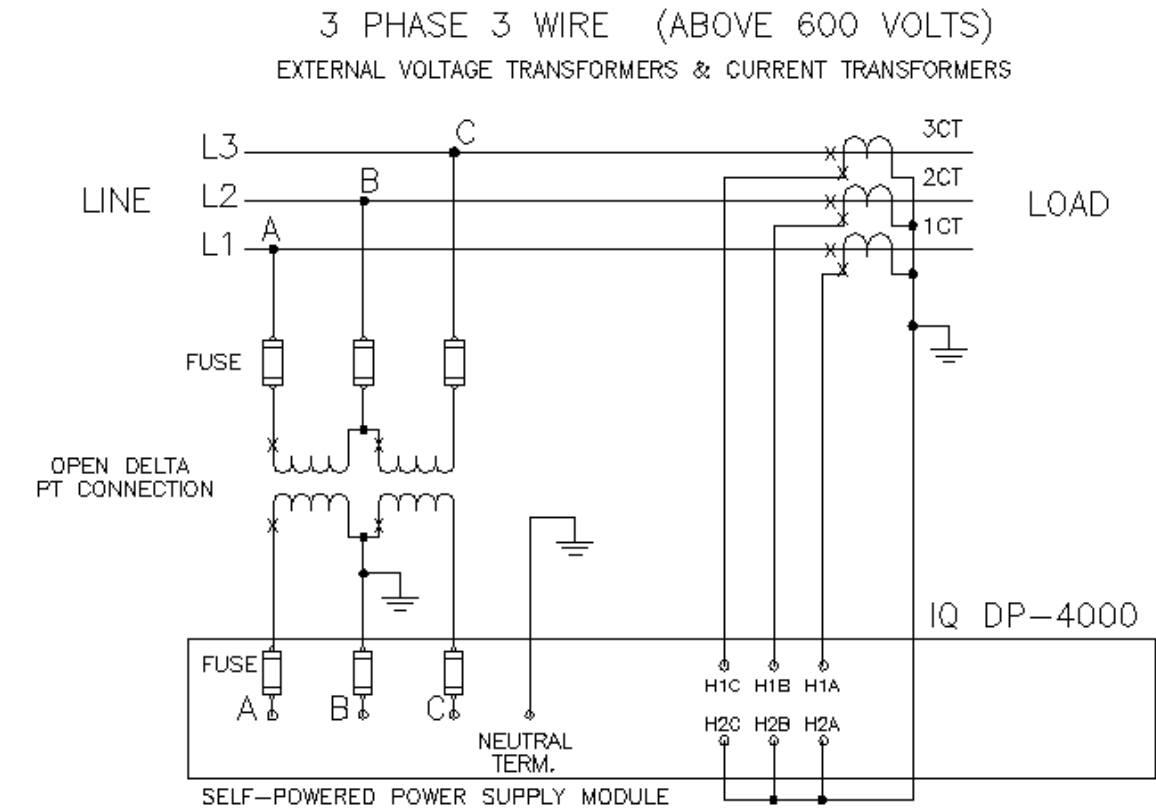
Figure 4.11 3-Phase, 3-Wire (above 600 volts) Wiring Diagram
