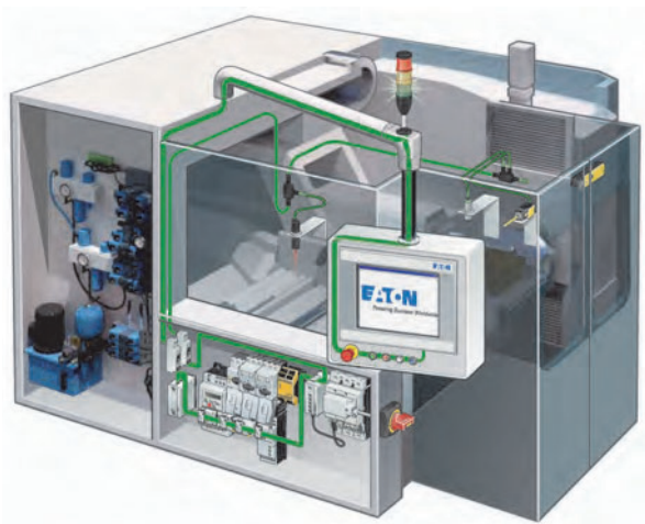
SmartWire-DT In Panel and On Machine Wiring Solution
