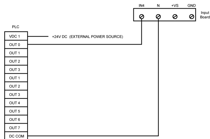
Figure 10: Connecting 24 V input board to a PLC. See Table 5
