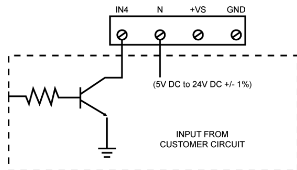
Figure 8: Wiring to 24 V input board with an open collector transistor
