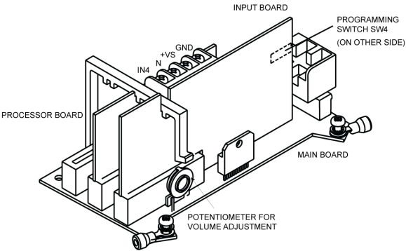
Figure 14: PC board locations
