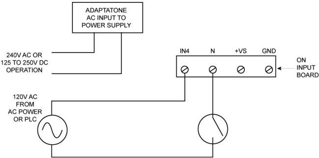
Figure 13: Connecting from a PLC to 120 V input board. See Table 5
