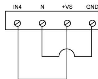
Figure 7: 24 VDC strapped input, 24 V input board
