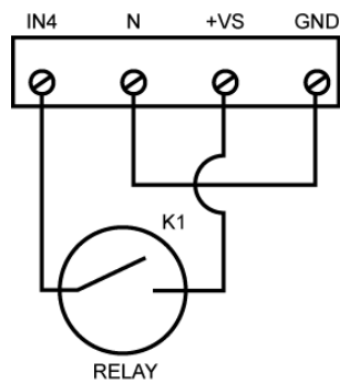
Figure 6: Wiring a dry relay contact to 24V input board, method 2
