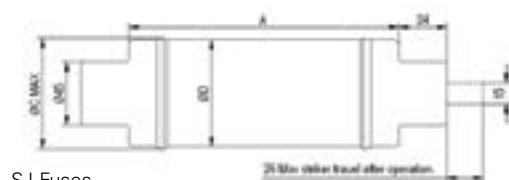
SJ Fuses
