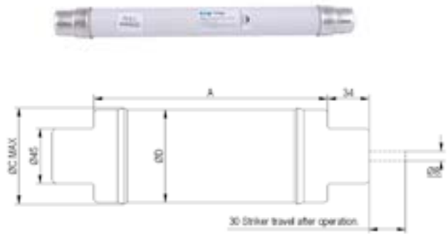
Dimensions - mm
