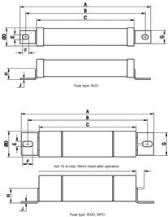
Tag type '6'
