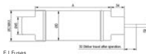
EJ Fuses
