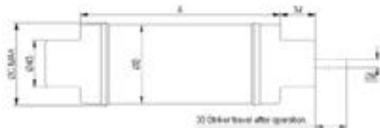
EJ Fuses
