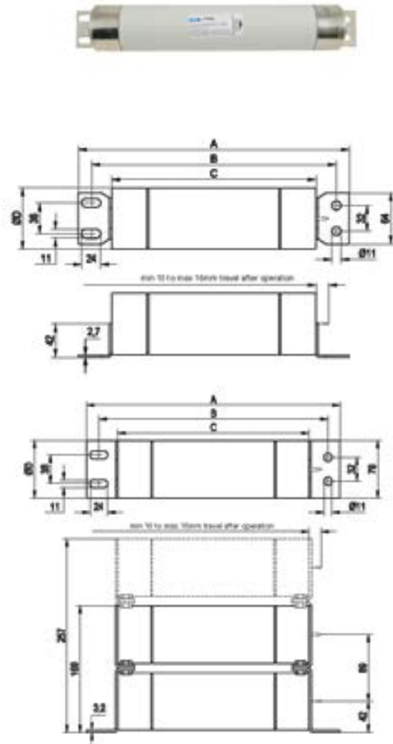
Triple barrel fuse link (3rd barrel shown dotted) with 03 tags. Double barrel fuse link with 02 tags shown in full line.
