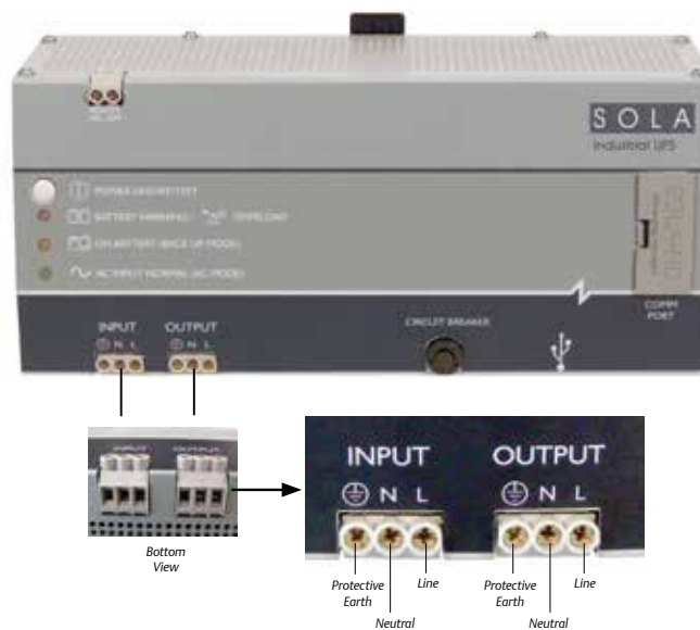
Figure 2: Input/Output Terminals
