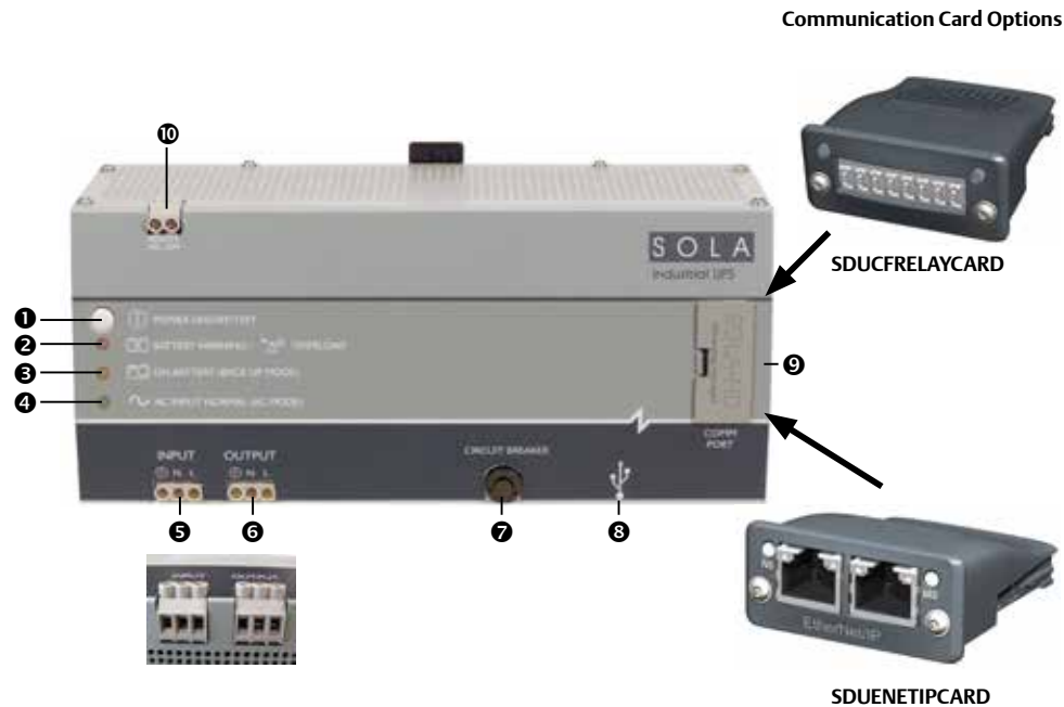
Figure 4: Front Panel
