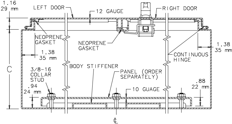
SECTION X-X
