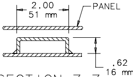
SECTION Z-Z
