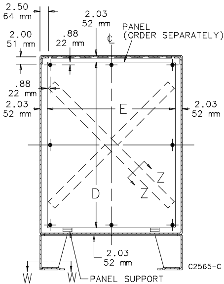
SECTION Y-Y
