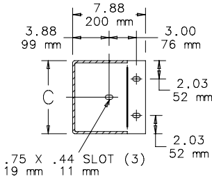
SECTION W-W
