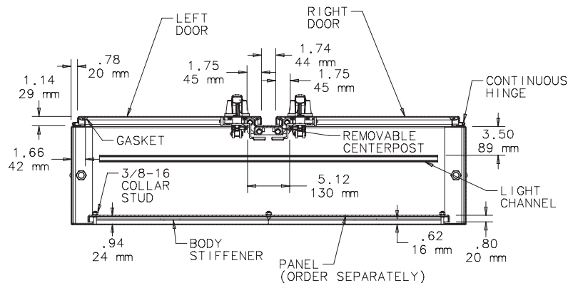
SECTION X-X
