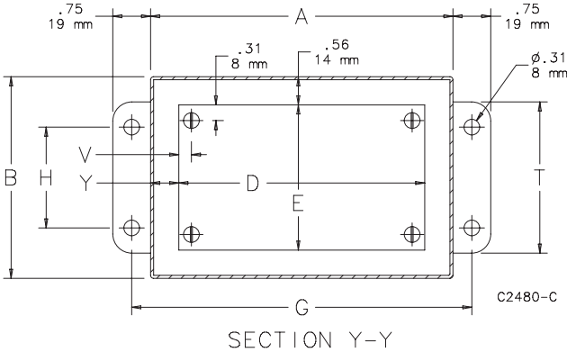
SECTION Y-Y
