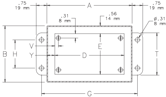
SECTION Y-Y
