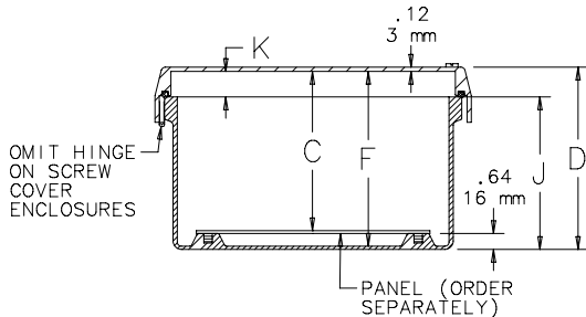
SECTION X-X
