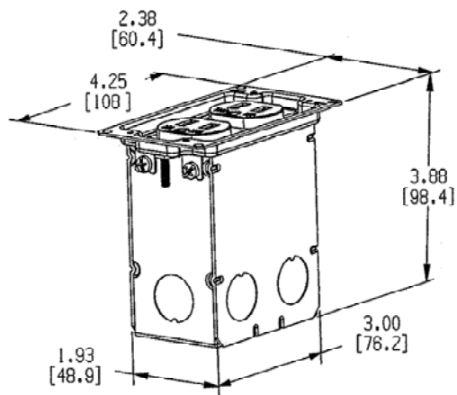
ISOMETRIC VIEW OF ASSEMBLED BOX, ADAPTOR & RECEPTACLE
