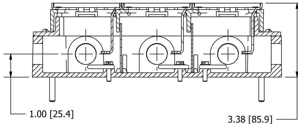
SECTION A-A THROUGH FLOOR BOX WITH COVER ASSEMBLY INSTALLED AT MAXIMUM HEIGHT.
