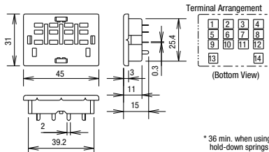
Terminal Arrangement
