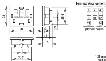
Terminal Arrangement
