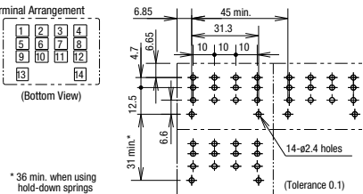
Terminal Arrangement
