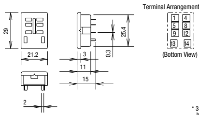
Terminal Arrangement
