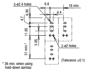
Terminal Arrangement
