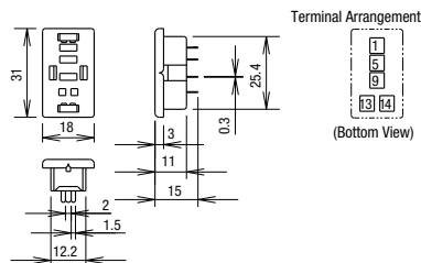
Terminal Arrangement
