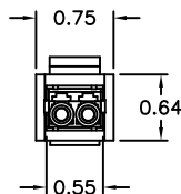
FRONT VIEW (DUST CAPS REMOVED)
