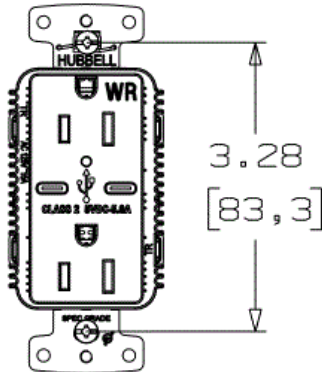
15A WEATHER RESISTANT (WR) DEVICE
