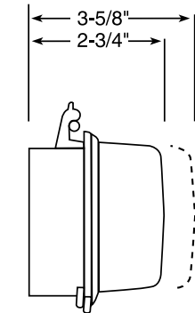
WP1100C, WP1110C
