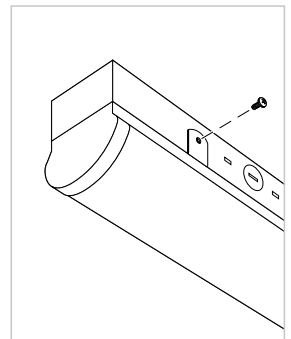
Swing the hanging lamp into position and secure brackets with screws.
