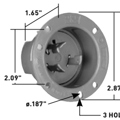
20A Flanged Inlet & Outlet
