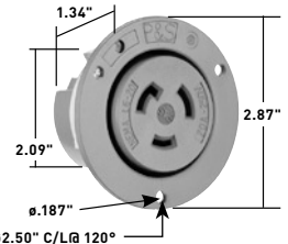
20A Flanged Inlet &amp; Outlet
