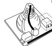
Encapsulated Core & Coil (73B Series)
