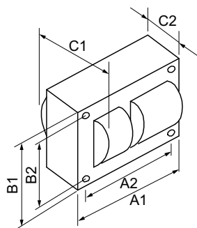
MH BAL 250W M138/M153 QUAD KIT
