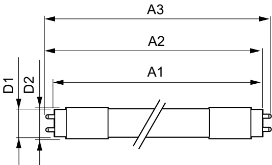
TLED 1200mm 120V 13-32W 2100lm 5000K G13
