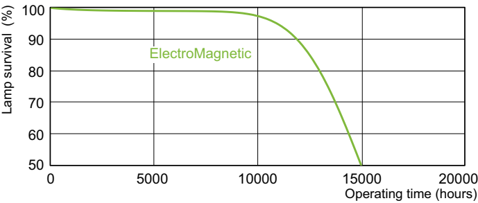
TL-D Standard Colours Life Expectancy 12 h cycle
