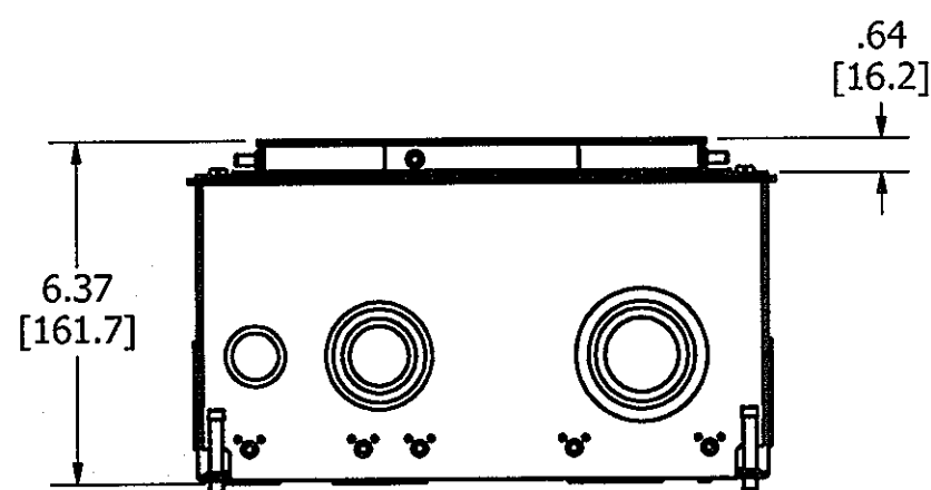
END VIEW
