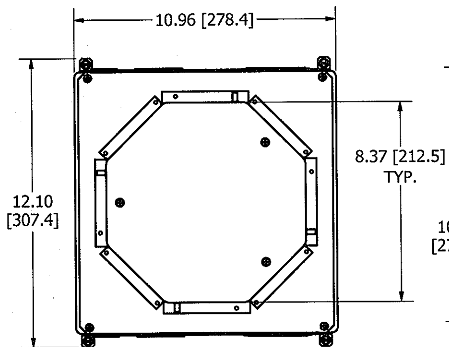
TOP VIEW
