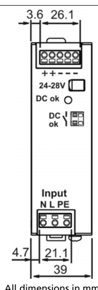
Fig. 22-3 Front view CP10.241-S2
