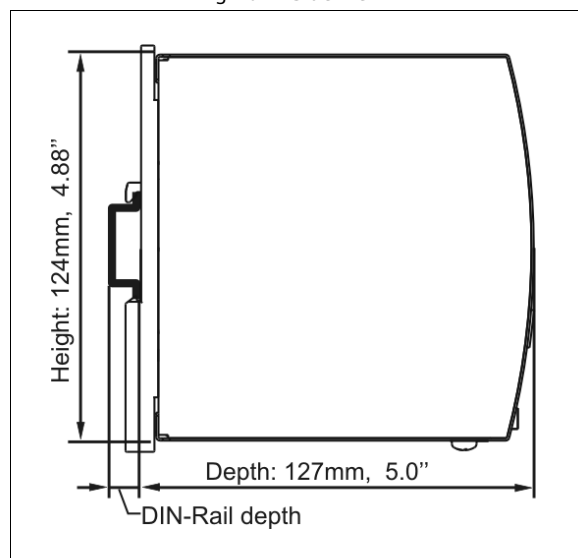
Fig. 20-2 Side view
