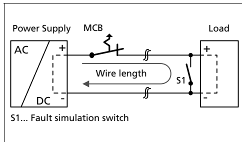
Fig. 21-5 Test circuit
