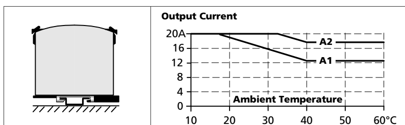
Fig. 21-8 Mounting Orientation C (Table-top mounting)
