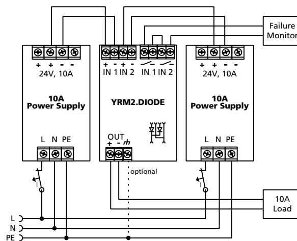
Fig. 18-1 Wiring diagram, 1+1 Redundancy, 10A output current
