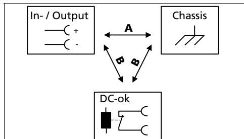
Fig. 14-1 Dielectric strength
