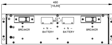
VIEW ROTATED 180°
