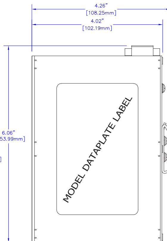
RIGHT SIDE
