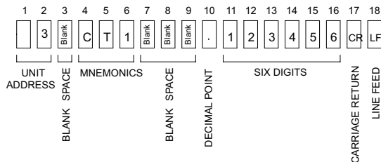
Figure 14, Transmission String
