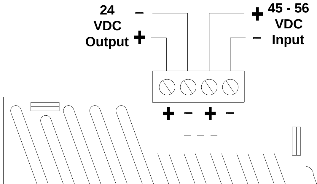
EB-PS-4824-13 Power Connections
