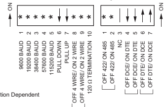
ICM5 DIP Switch Settings
