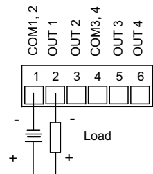
Solid State NFET Version
