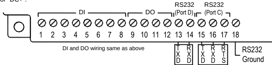
VT-UIPM-441 with 8 DI, 4 DO, 1 RS485 & 3 RS232
