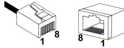
RJ45 Connectors
