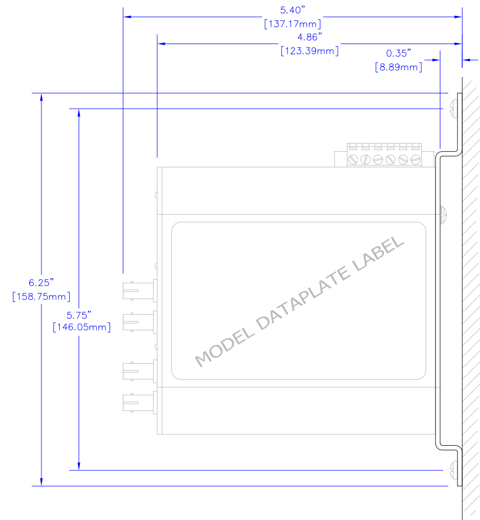
OPTIONAL COMPACT PANEL MOUNT ASSY. ( P/N: CPMA-1 )
