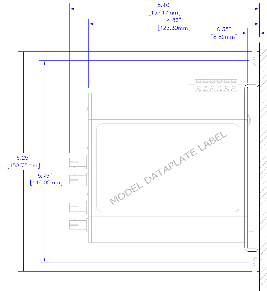
OPTIONAL COMPACT PANEL MOUNT ASSY. ( P/N: CPMA-2 )
