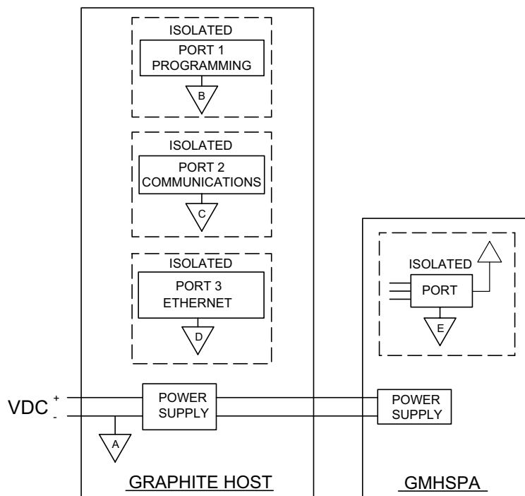
Block Diagram for GMHSPA
